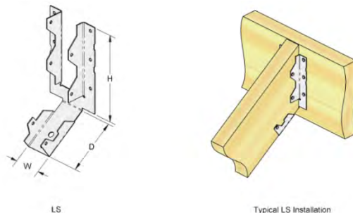
FIGURE 1—LS LIGHT SLOPE HANGER
