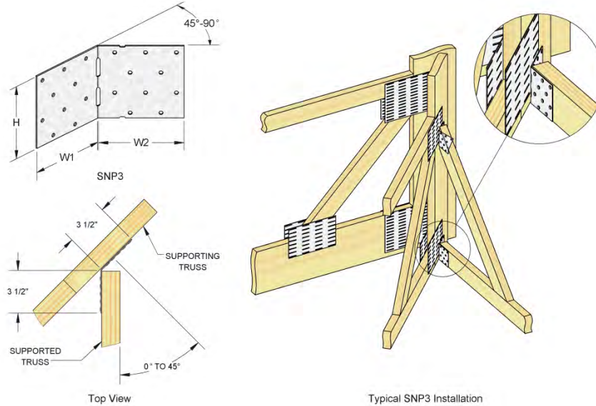
FIGURE 5—DIMENSIONS AND INSTALLATION OF SNP SKEWABLE NAILER PLATE
