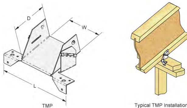
FIGURE 6—TMP RAFTER-TO-PLATE CONNECTOR
